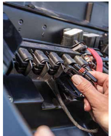
CREW XP 1000 POLARIS PULSE WIRING SHOWN
