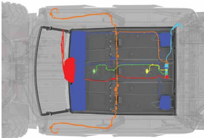
CREW XP 1000 POLARIS PULSE WIRING SHOWN
